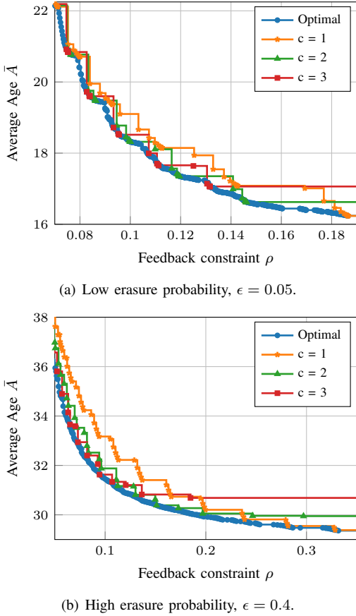
Fig. 4: Performance of periodic hybrid ARQ schemes compared to optimal allocations when using random linear codes with N = 30 , K = 10
