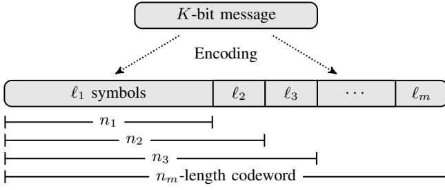
Fig. 2: In a hybrid ARQ scheme, a K -bit source message is encoded into a N -length codeword. The codeword is further divided into sub-blocks of varied lengths, which are sequentially transmitted up to an ACK message from the receiver.
